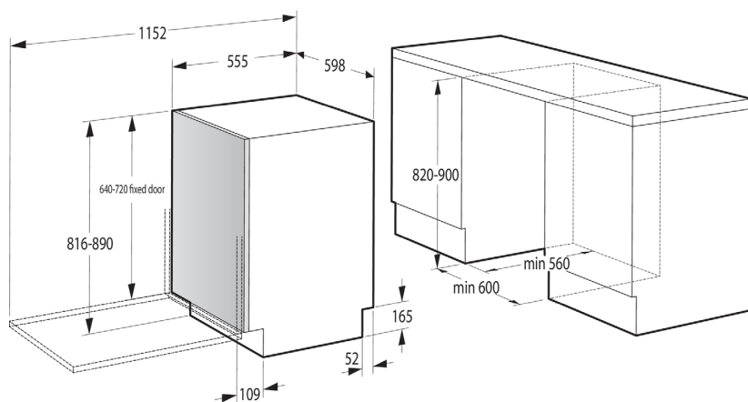
Gorenje | GV642C65 / GV663A66
