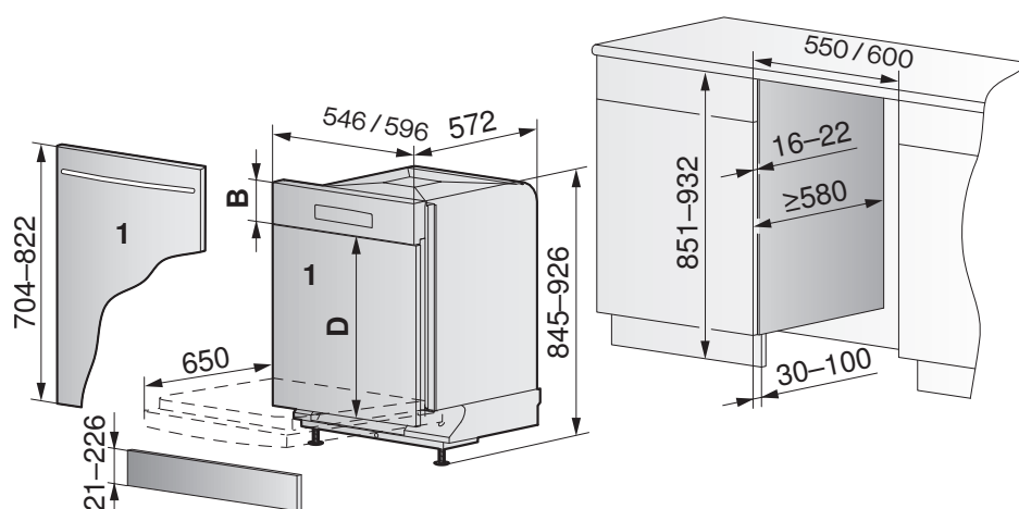
SIBIR | GS 55 V 2000 (Grand volume) / GS 60 V 2000 (Grand volume)
