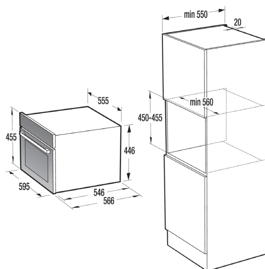
Gorenje | BCM 4058 B
