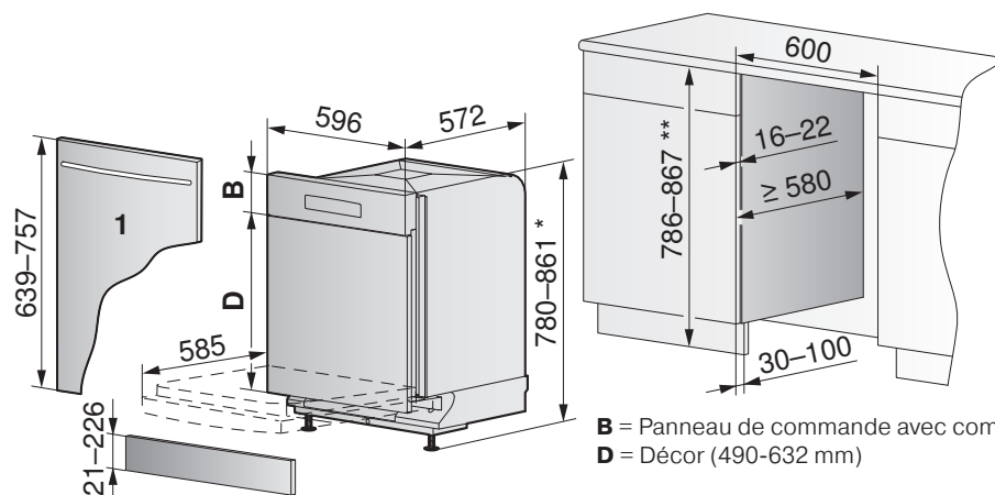
SIBIR | GS 60 V 4000 / GS 60 V 2000
