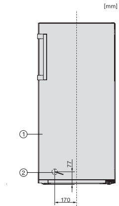
FN4712E, installation (footnote*) (installation drawings)
