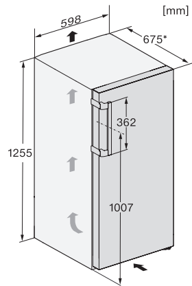
FN4712E, installation sketch (footnote*) (installation drawings)
