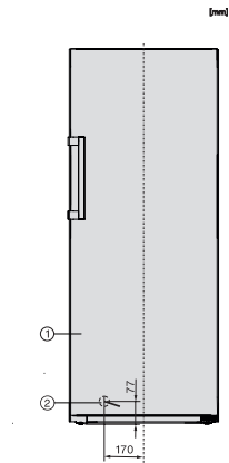
FN4748D, installation (footnote*) (installation drawings)
